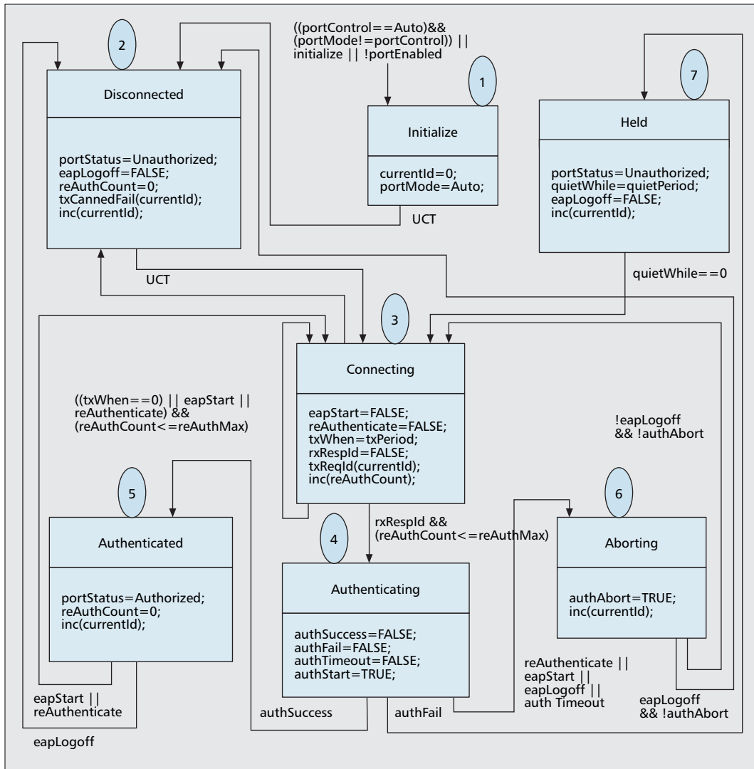
Figure 4. PAE state machine in authenticator.
